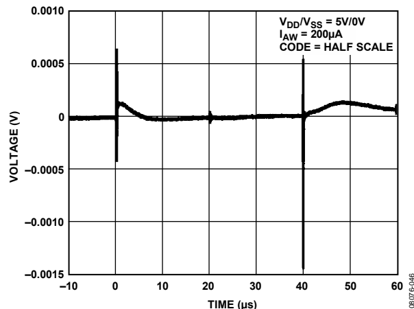
Figure 34. Digital Feedthrough
