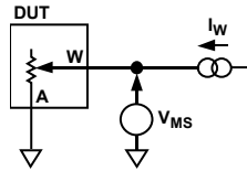
Figure 38. Resistor Position Nonlinearity Error (Rheostat Operation; R-INL, R-DNL)
