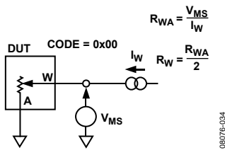
Figure 39. Wiper Resistance
