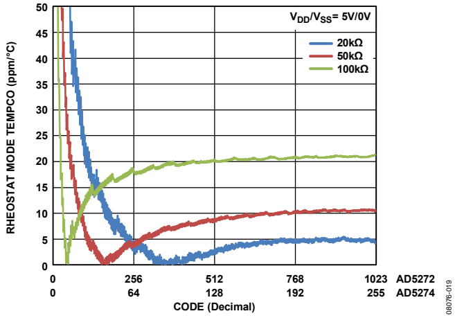
Figure 24. Tempco \Delta R_{w}/\Delta T vs. Code
